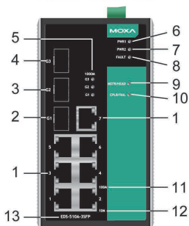
EDS-510A-3SFP Front Panel View
